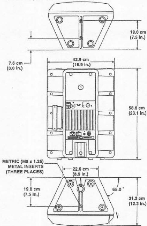
FIGURE 2 — Sx200a Dimensions
